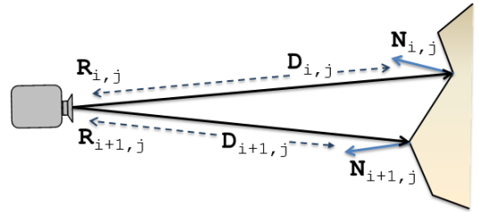
Figure 6: Updated gradients can be computed based on neighboring ray directions, estimated depth and surface normals.
